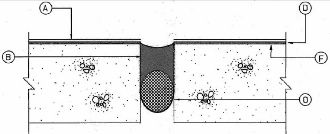
EXPANSION JOINTS GREATER THAN 1/2"
