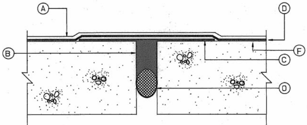
EXPANSION JOINTS UP TO 1/2"
